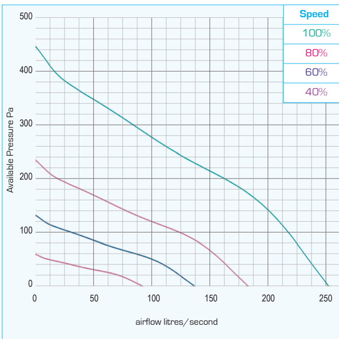
Purge-Box 200
